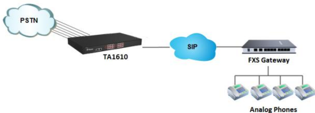
Figure 2-3 Connect TA FXO Gateway and FXS Gateway
