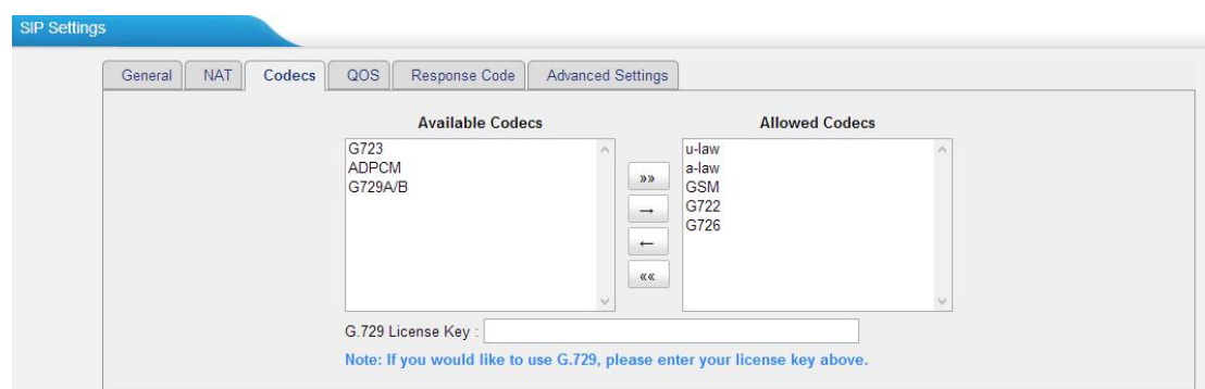
Figure 4-8 Codecs
