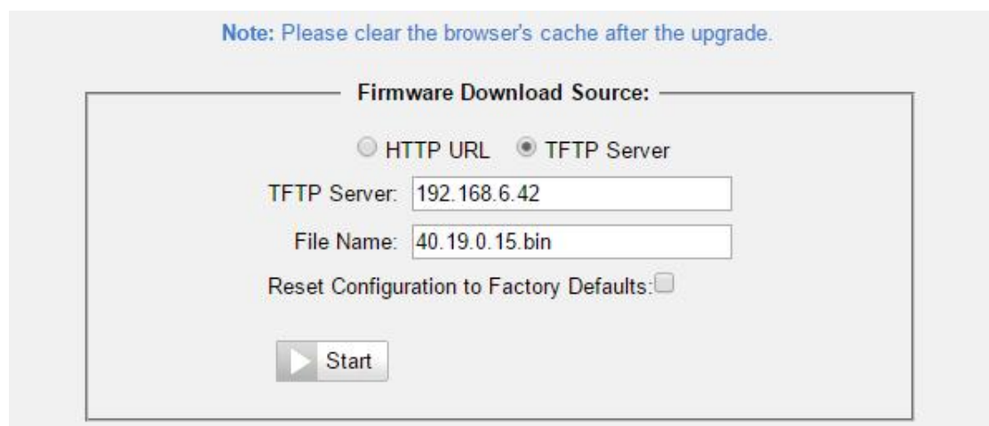
Figure 11-10 Upgrade through HTTP
